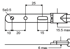
Metal clip dimension for Type J
