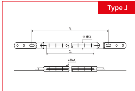
Metal clip dimension for Type J
